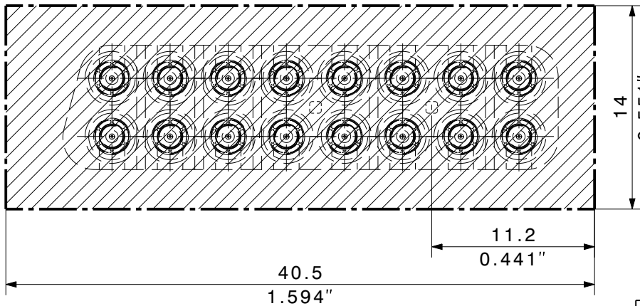
Mounting hole
