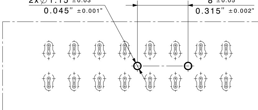
Mounting hole
